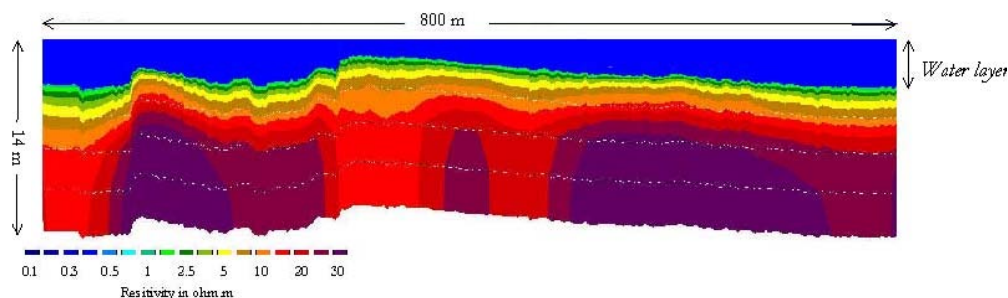
Inversed Resistivity section (3000 data points in 10 minutes)
